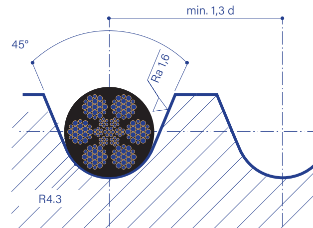
Specified Groove Diagram for CTP® 8.1 mm
