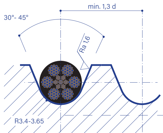
Specified Groove Diagram for CTP® 6.5 mm
